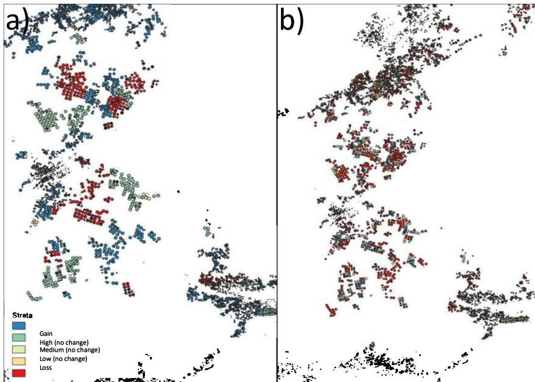
Figure 18. Classification of clusters based on the a) Landsat Normalized Difference Vegetation Index (NDVI) and b) actual evapotranspiration
